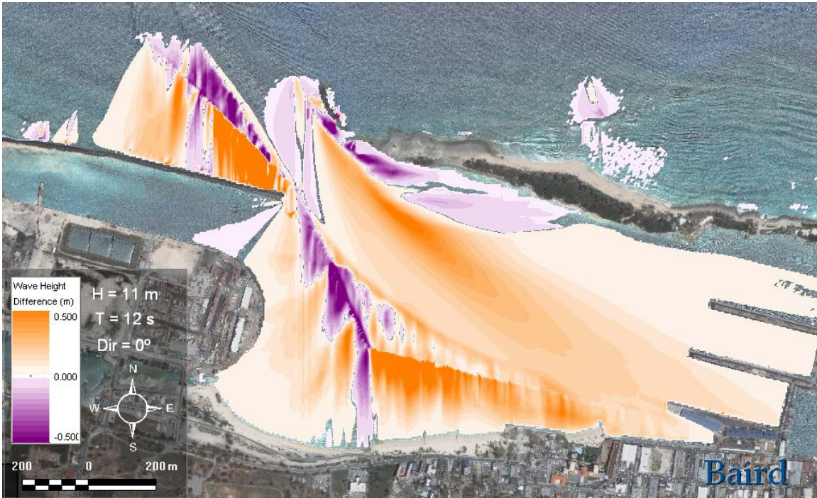
Figure D-7 Wave height difference plot inside the harbor for N hurricane waves.
