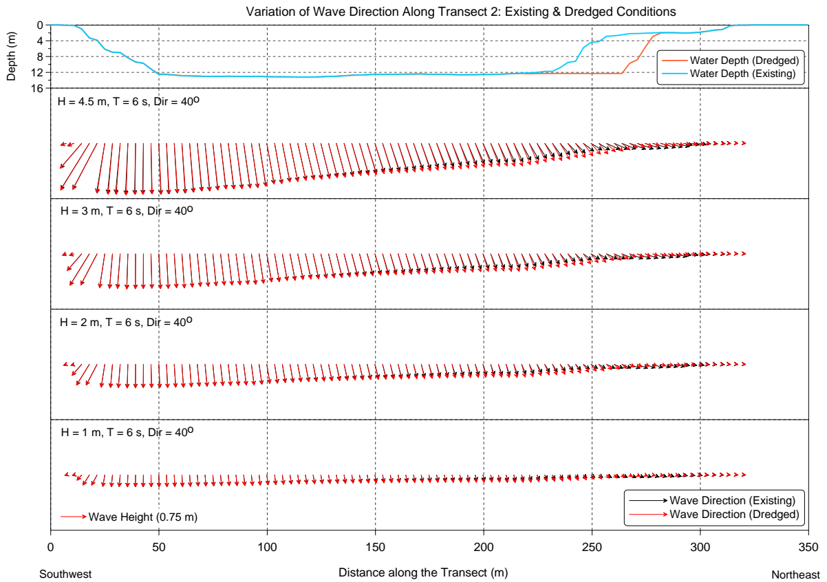
Figure E-16 Wave height vector comparisons along Transect 2 for 6 s, NE waves.
