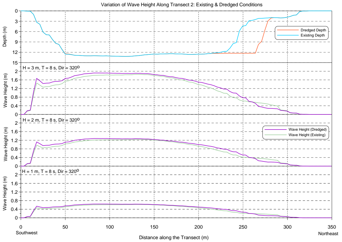
Figure E-21 Wave height comparisons along Transect 2 for 8 s, NW waves.
