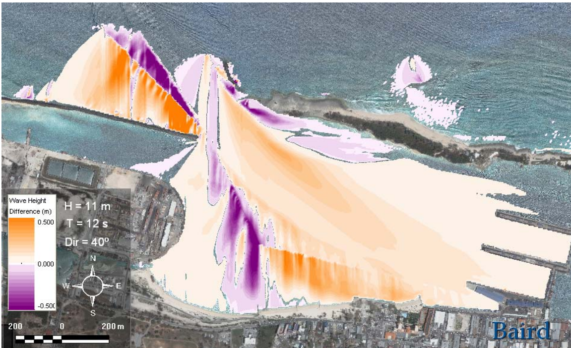
Figure D-8 Wave height difference plot inside the harbor for NE hurricane waves.
