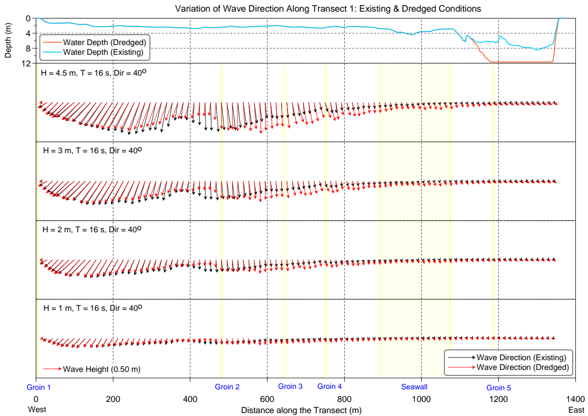
Figure E-8 Wave height vector comparisons along Transect 1 for 16 s, NE waves.
