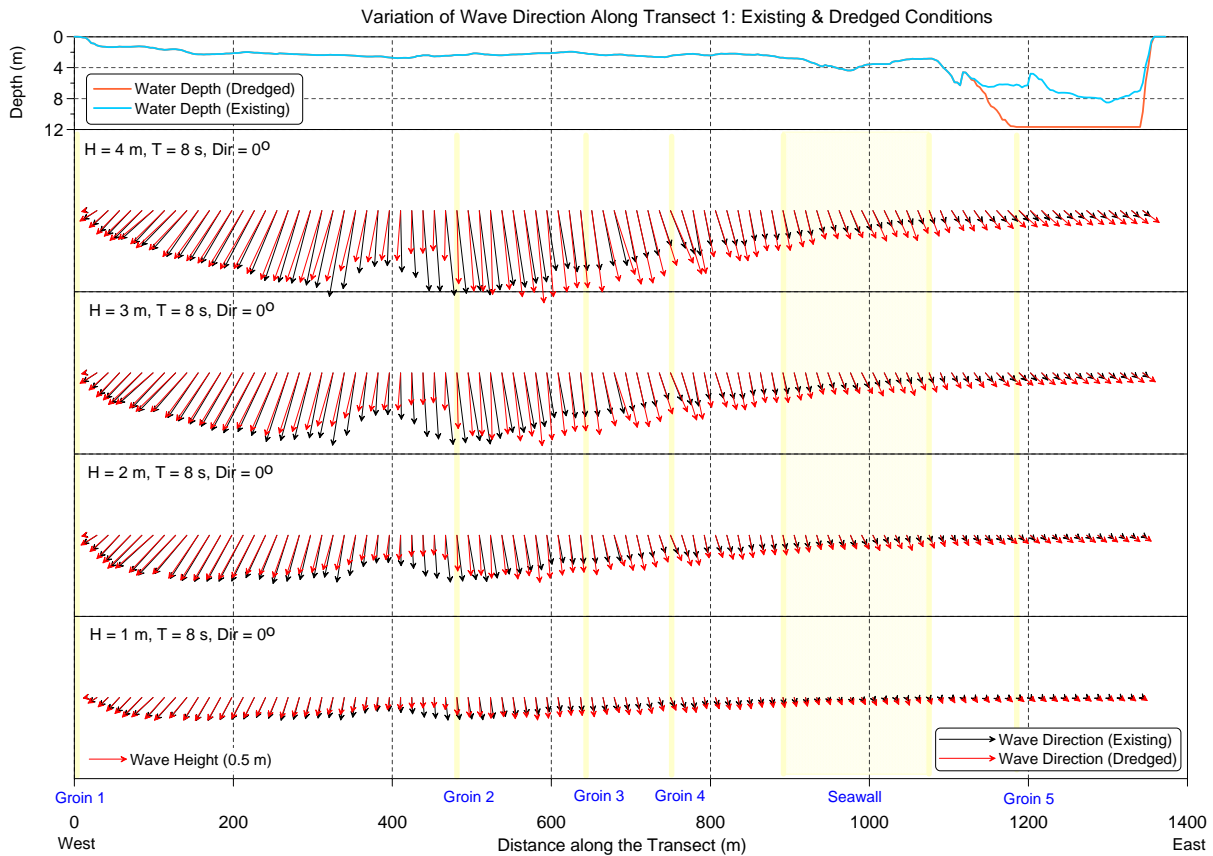
Figure E-2 Wave height vector comparisons along Transect 1 for 8 s, N waves.
