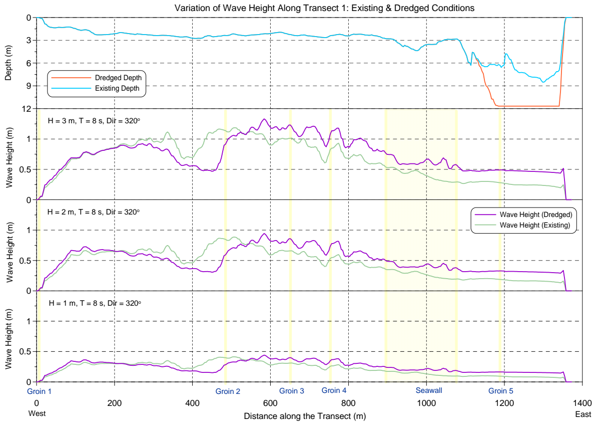
Figure E-9 Wave height comparisons along Transect 1 for 8 s, NW waves.
