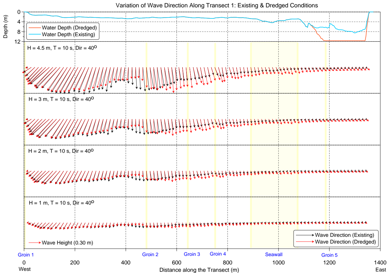
Figure E-6 Wave height vector comparisons along Transect 1 for 10 s, NE waves.
