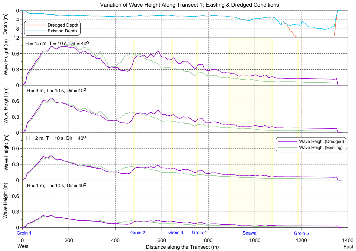
Figure E-5 Wave height comparisons along Transect 1 for 10 s, NE waves.
