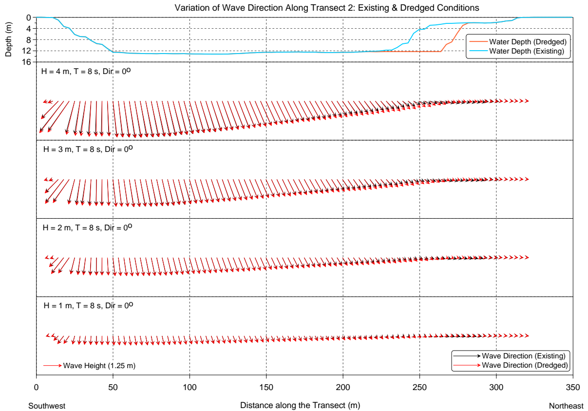
Figure E-14 Wave height vector comparisons along Transect 2 for 8 s, N waves.
