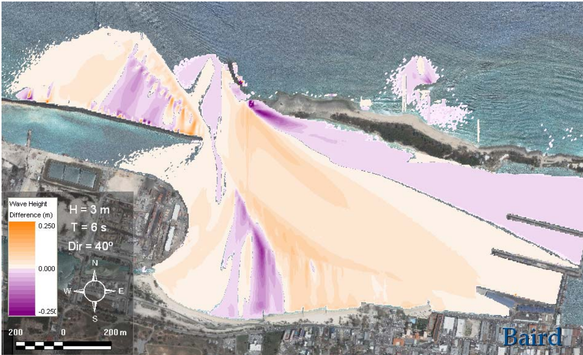
Figure D-3 Wave height difference plot for 3 m, 6 s, NE waves.
