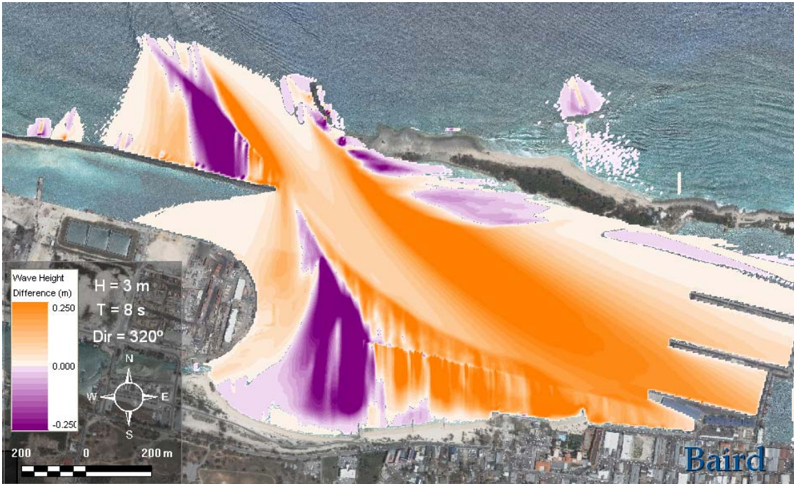
Figure D-1 Wave height difference plot for 3 m, 8 s, NW waves.
