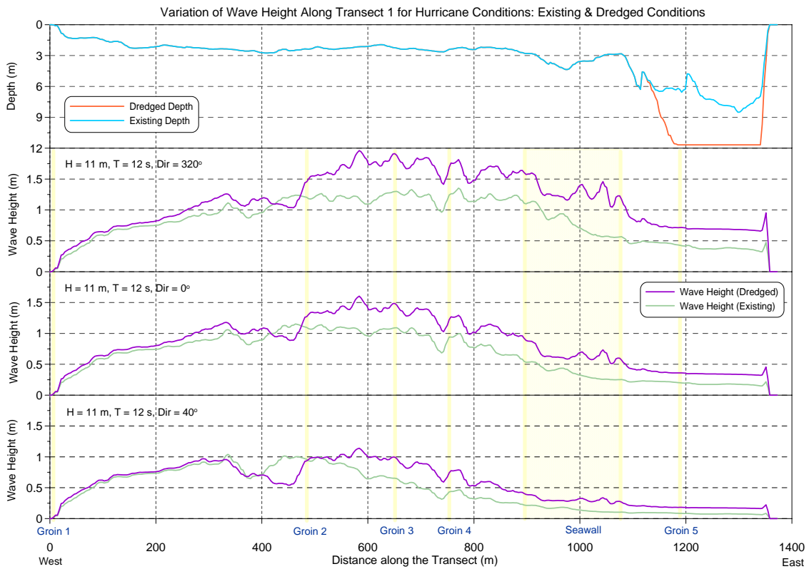
Figure E-11 Wave height comparisons along Transect 1 for 12 s, N waves.
