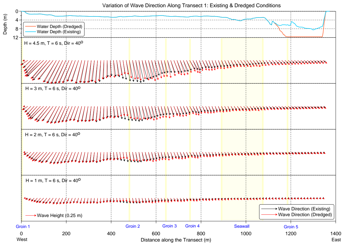
Figure E-4 Wave height vector comparisons along Transect 1 for 6 s, NE waves.
