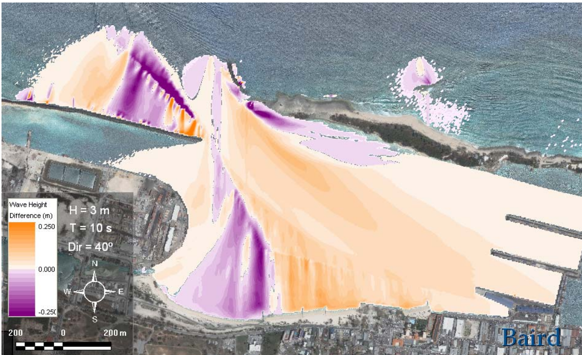
Figure D-4 Wave height difference plot for 3 m, 10 s, NE waves.
