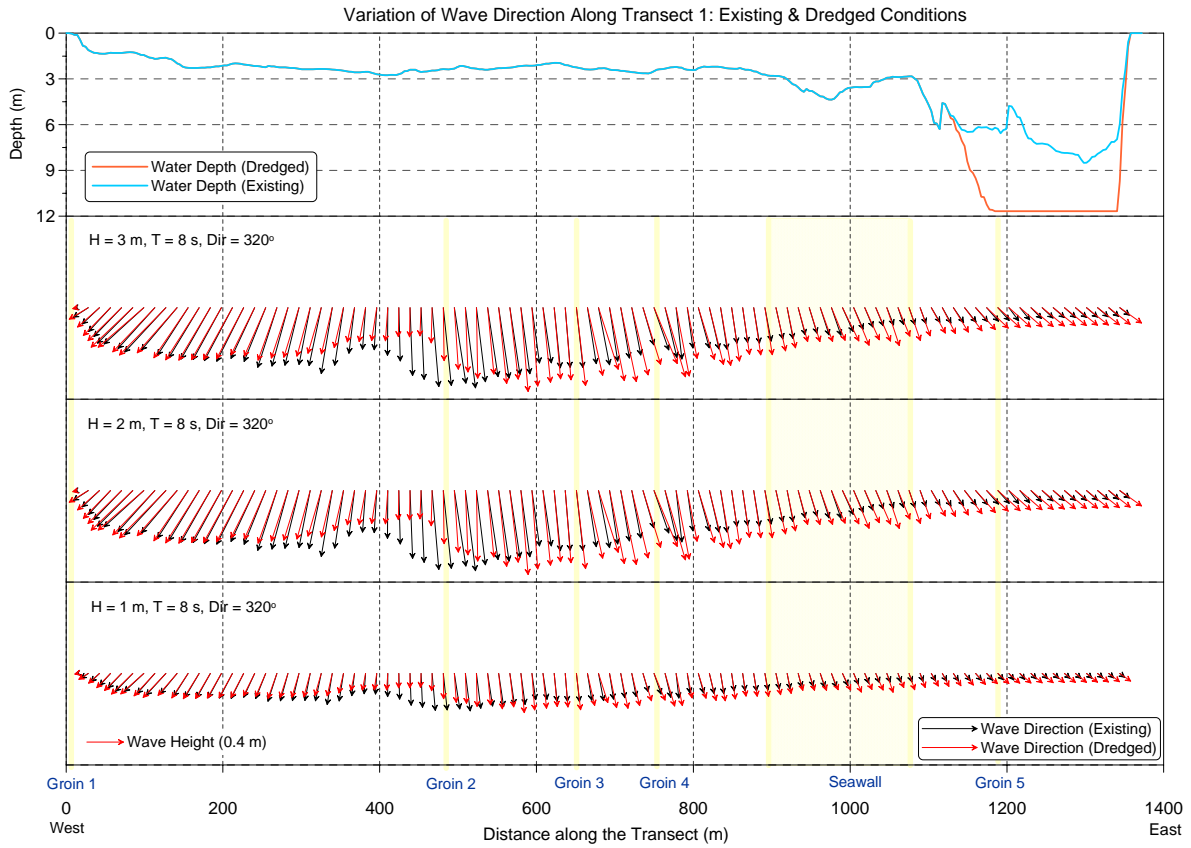
Figure E-10 Wave height vector comparisons along Transect 1 for 8 s, NW waves.
