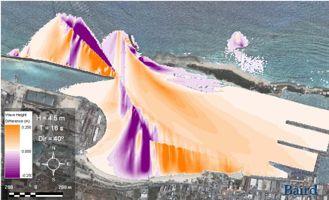
Figure D-5 Wave height difference plot for 4.5 m, 16 s, NE waves.
