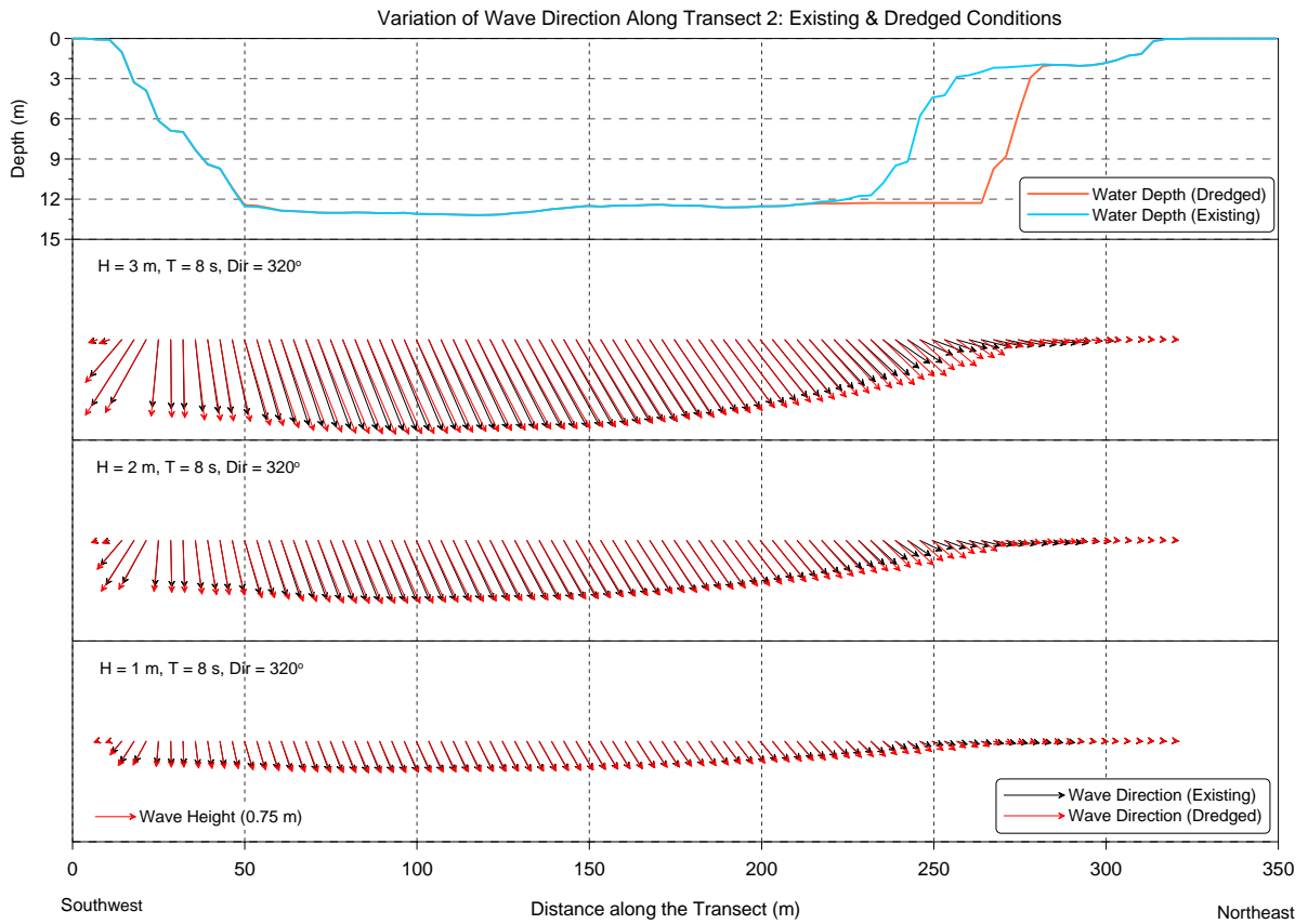
Figure E-22 Wave height vector comparisons along Transect 2 for 8 s, NW waves.
