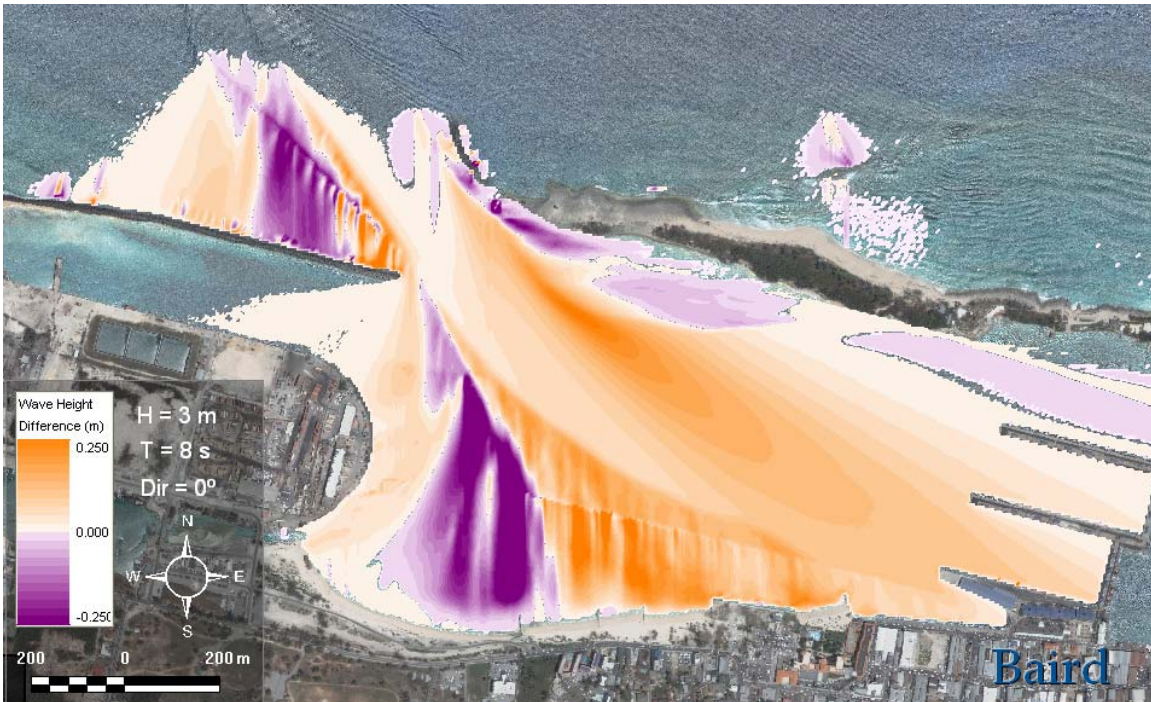
Figure D-2 Wave height difference plot for 3 m, 8 s, N waves.
