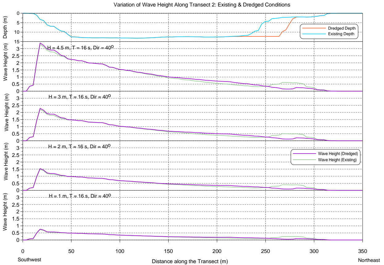
Figure E-19 Wave height comparisons along Transect 2 for 16 s, NE waves.
