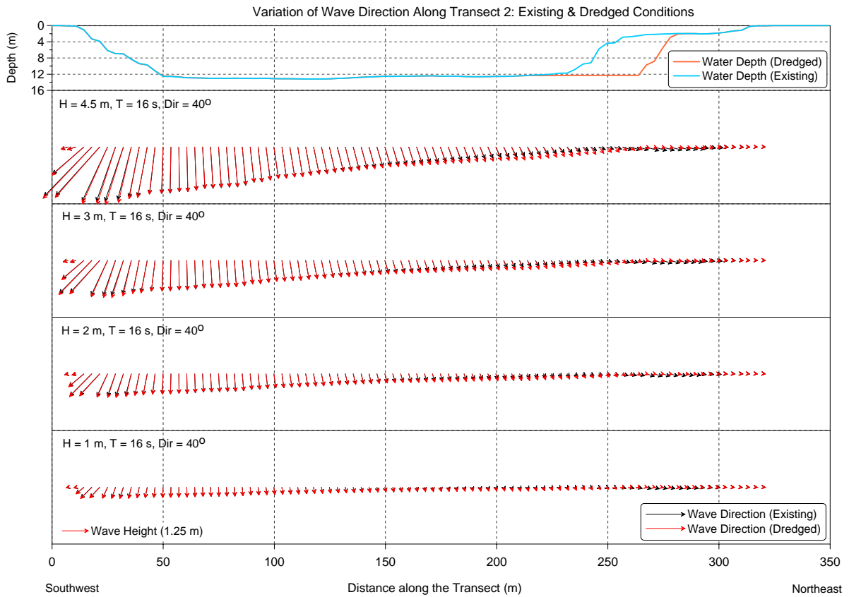
Figure E-20 Wave height vector comparisons along Transect 2 for 16 s, NE waves.
