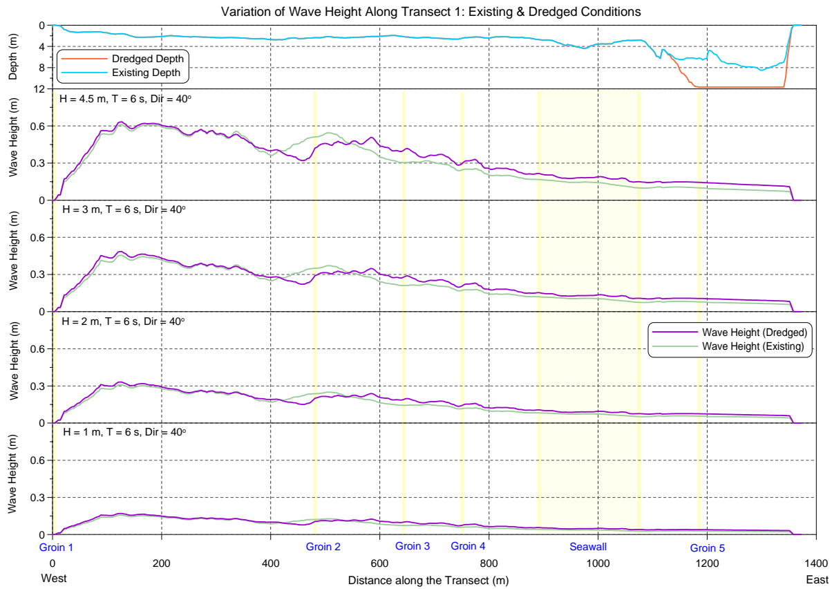
Figure E-3 Wave height comparisons along Transect 1 for 6 s, NE waves.
