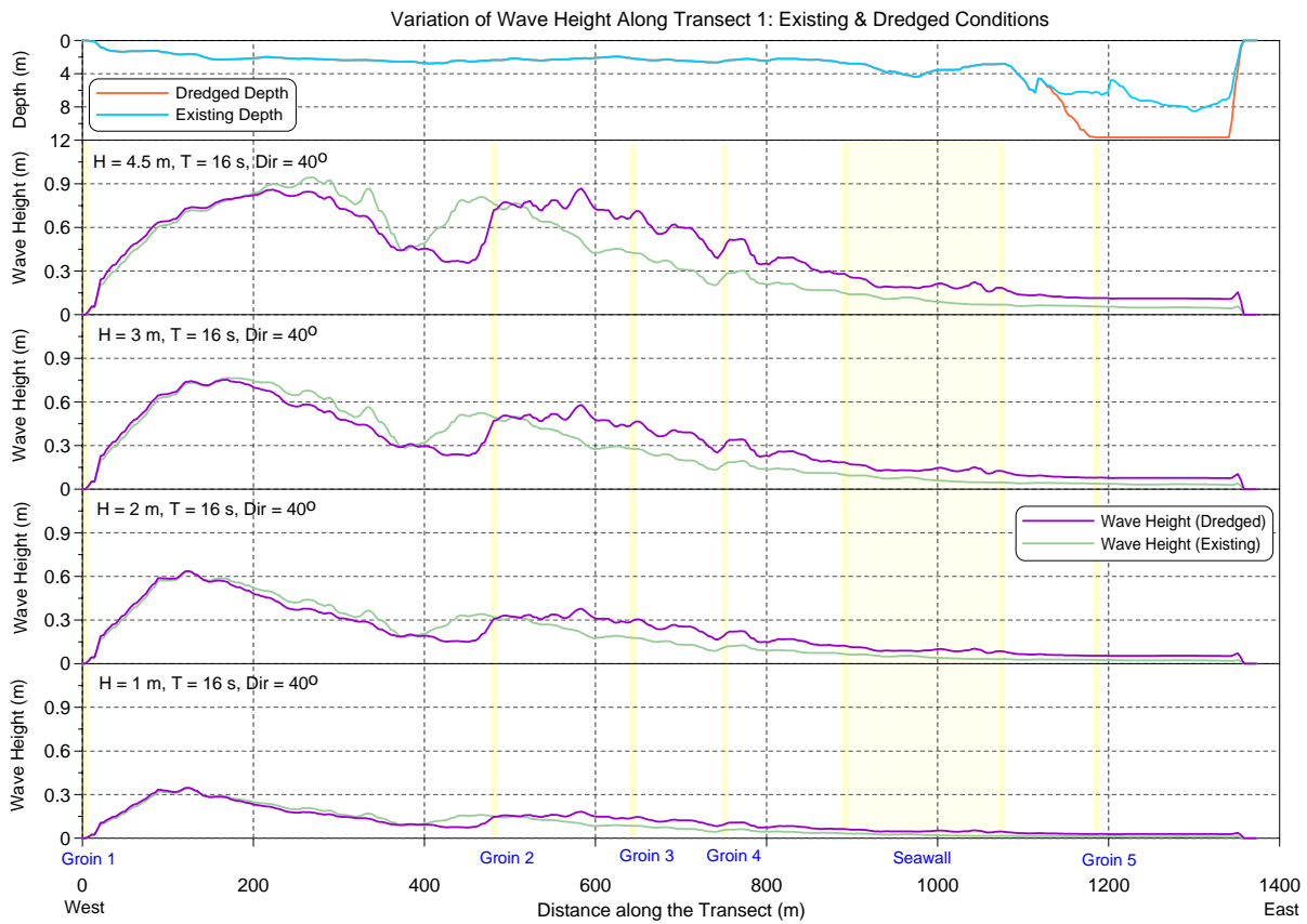
Figure E-7 Wave height comparisons along Transect 1 for 16 s, NE waves.
