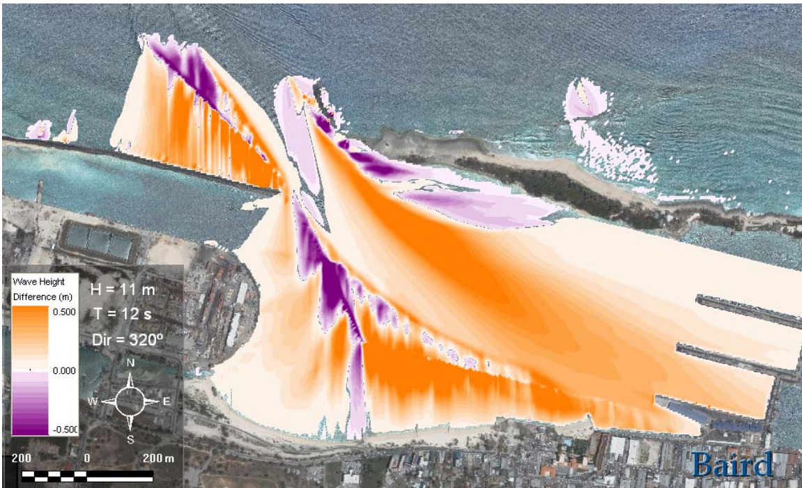
Figure D-6 Wave height difference plot for 11 m, 12 s, NW waves.
