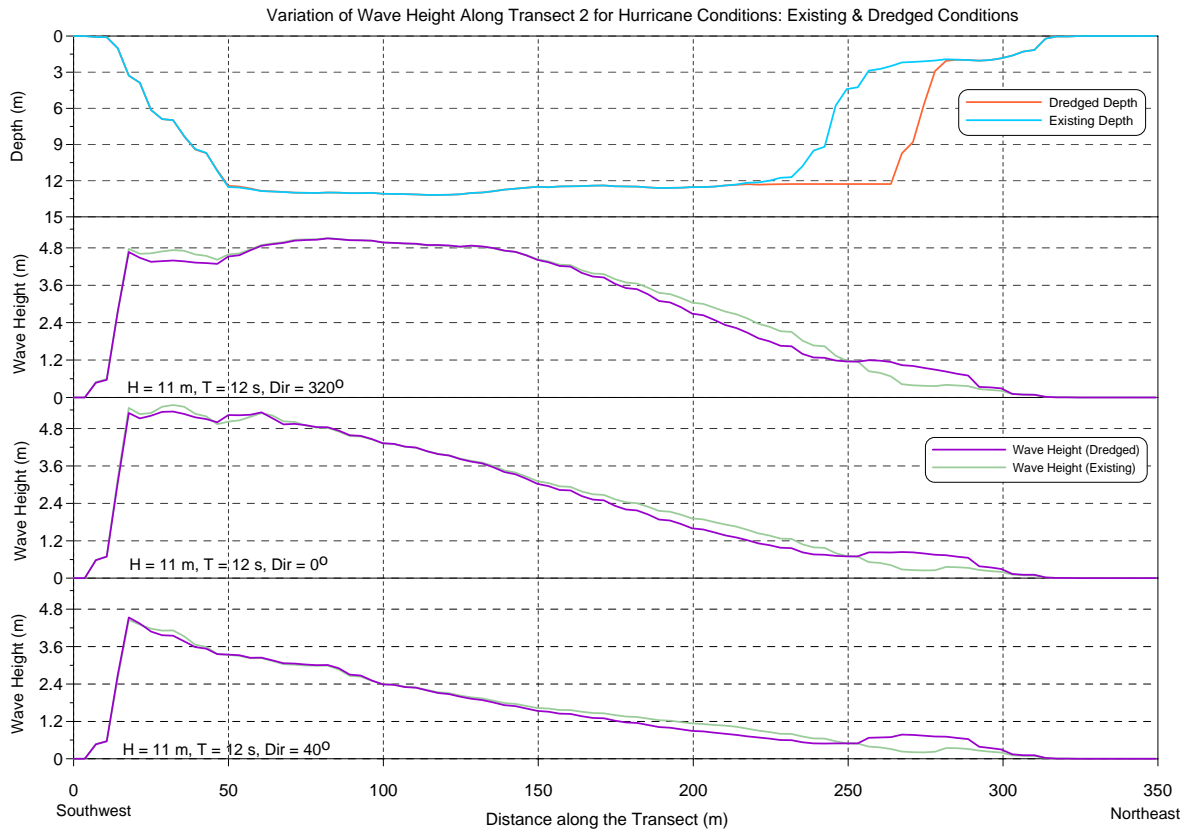
Figure E-23 Wave height comparisons along Transect 2 for 12 s, N waves.
