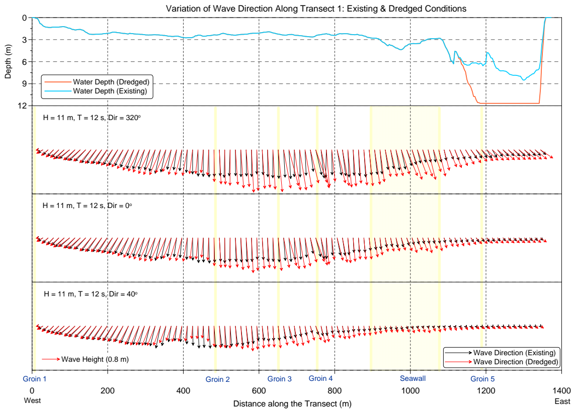
Figure E-12 Wave height vector comparisons along Transect 1 for 12 s, N waves.
