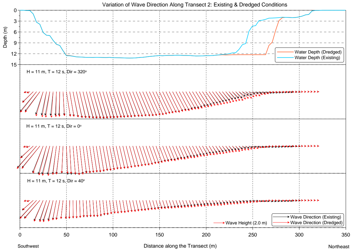
Figure E-24 Wave height vector comparisons along Transect 2 for 12 s, N waves.
