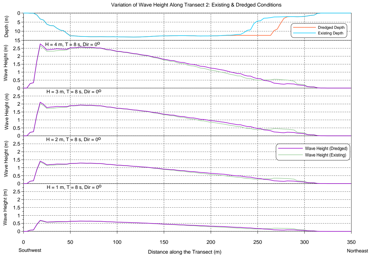
Figure E-13 Wave height comparisons along Transect 2 for 8 s, N waves.
