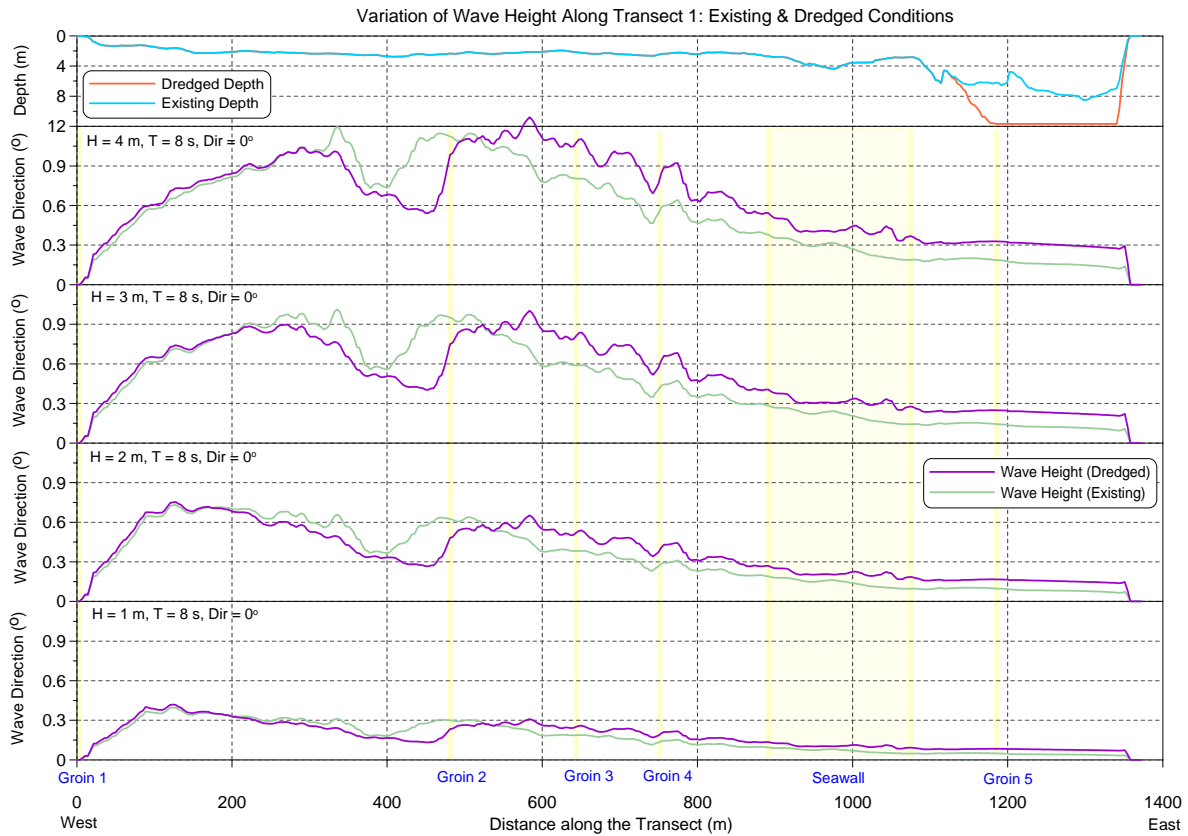
Figure E-1 Wave height comparisons along Transect 1 for 8 s, N waves.
