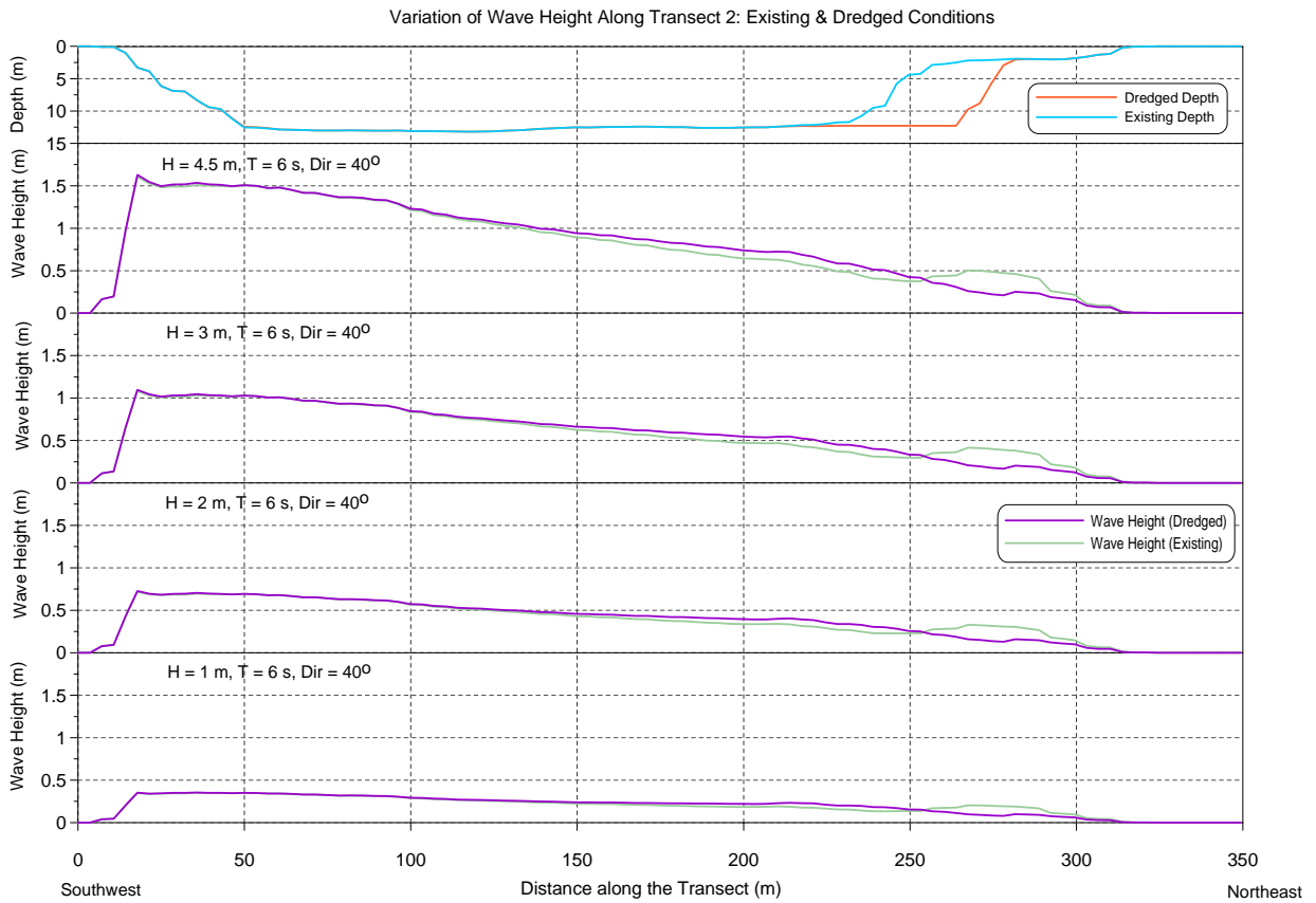
Figure E-15 Wave height comparisons along Transect 2 for 6 s, NE waves.
