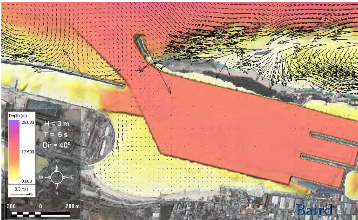
Figure C-3 Wave Heights (top) and Nearshore Currents (bottom) for 3 m, 6 s NW waves, Proposed Dredging
