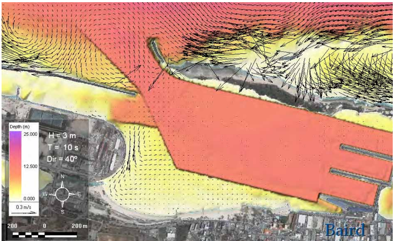
Figure C-4 Wave Heights (top) and Nearshore Currents (bottom) for 3 m, 10 s NE waves, Proposed Dredging
