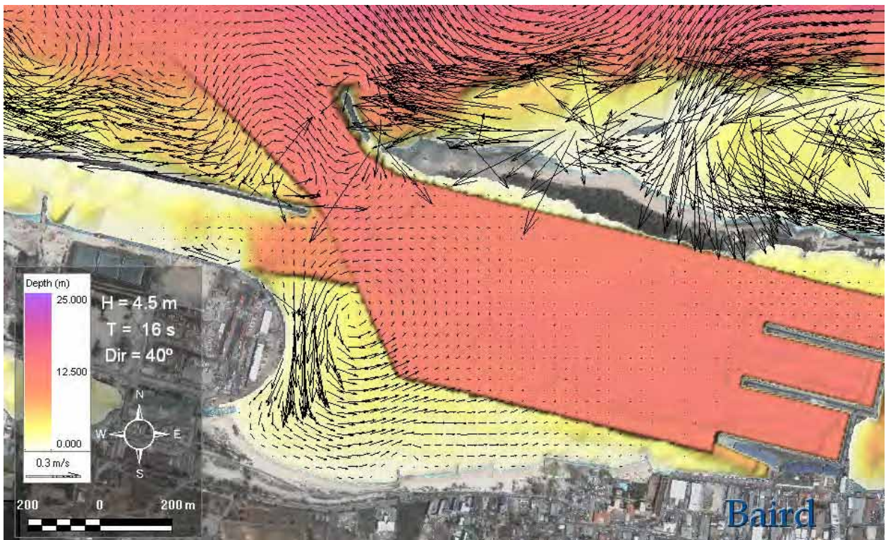
Figure C-5 Wave Heights (top) and Nearshore Currents (bottom) for 4.5 m, 16 s NE waves, Proposed Dredging
