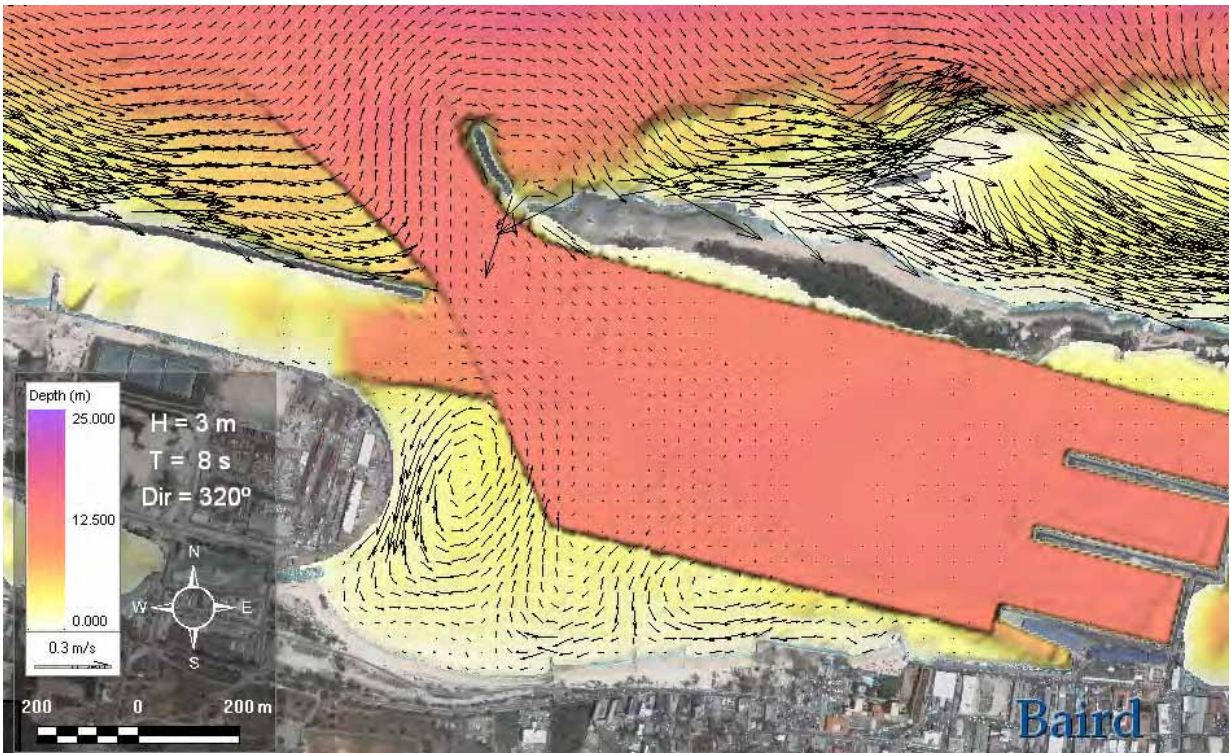
Figure C-1 Wave Heights (top) and Nearshore Currents (bottom) for 3 m, 8 s NW waves, Proposed Dredging
