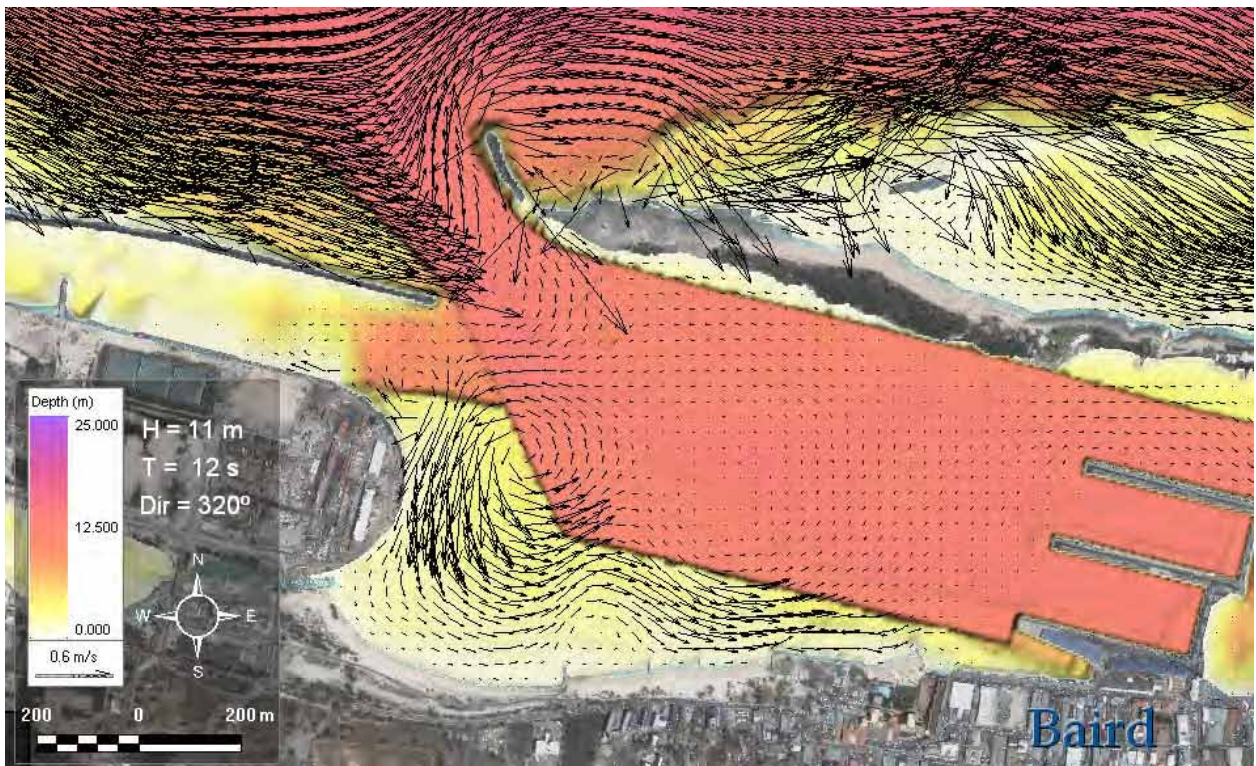
Figure C-6 Wave Heights (top) and Nearshore Currents (bottom) for 11 m, 12 s NW waves, Proposed Dredging
