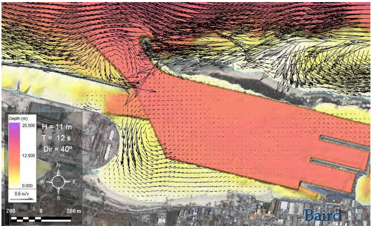
Figure C-8 Wave Heights (top) and Nearshore Currents (bottom) for 11 m, 12 s NE waves, Proposed Dredging
