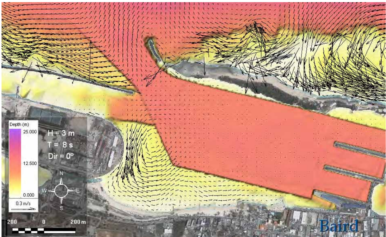
Figure C-2 Wave Heights (top) and Nearshore Currents (bottom) for 3 m, 8 s N waves, Proposed Dredging
