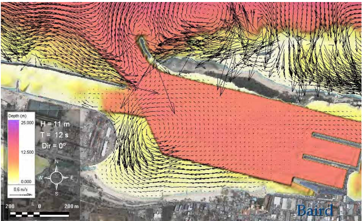
Figure C-7 Wave Heights (top) and Nearshore Currents (bottom) for 11 m, 12 s N waves, Proposed Dredging
